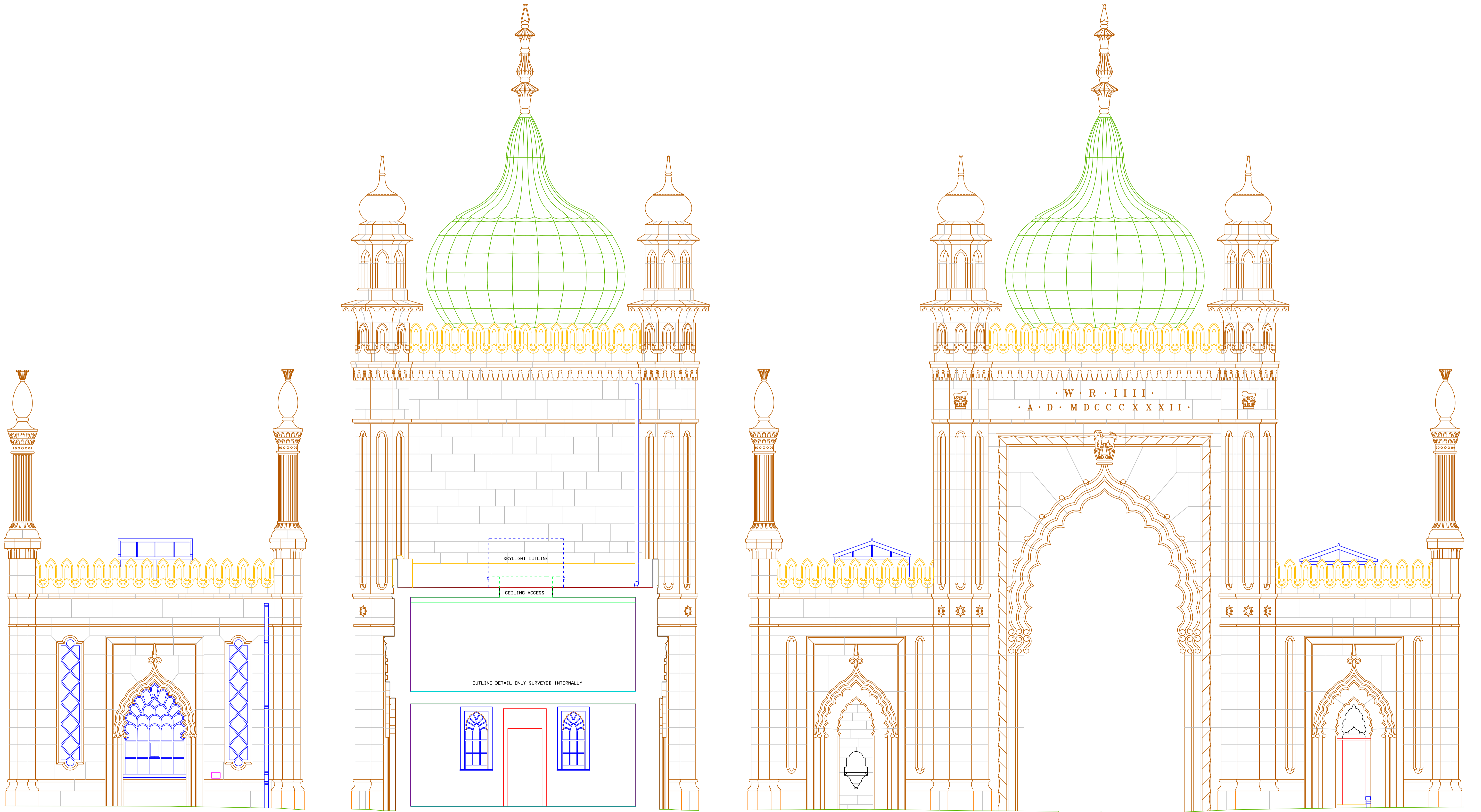
EAST LOWER ELEVATION
